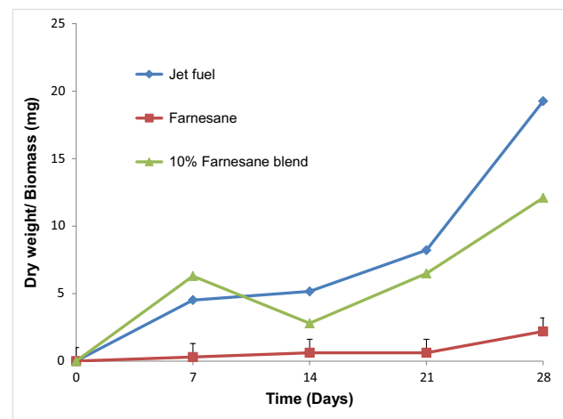
Fig. 1 Biomass values (mg) from the interface oil- aqueous phase at 0, 7, 14, 21, and 28 days for jet fuel, farnesane, and 10% farnesane blend samples with Hormoconis resiniae inoculum
